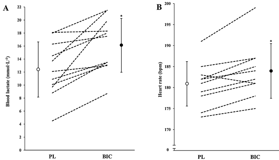
Fig. 1. Effect of sodium bicarbonate intake on blood lactate following and peak heart rate during a 90-s all out performance. Individual data points (n = 10–11) representing blood lactate (A) and peak heart rate (B). Participants first participated in a 3-h simulated cycling race. Immediately after, they performed a 90-sec all-out exercise bout. The participants received either oral sodium bicarbonate (BIC) or placebo (PL) supplements from baseline until the end of the 3-h cycling race. *P < 0.05 compared with PL.
