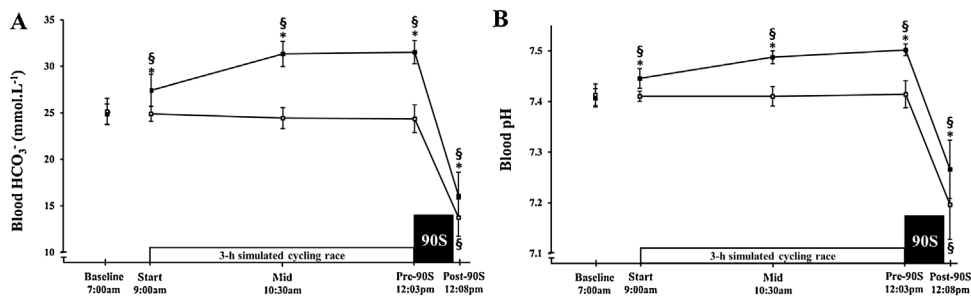
Fig. 3. Effects of sodium bicarbonate intake on blood acid-base balance. Data are mean ± SD (n = 11) for blood bicarbonate ( \text{HCO}_3^- ) (A) and blood pH (B) at baseline and at the start, middle, and end of a 3-h simulated cycling race, followed by a 90-s all-out exercise bout (90S). Participants received either oral sodium bicarbonate (■) or placebo (□) from baseline until the end of the 3-h race. *P < 0.05 compared with PL. §P < 0.05 compared with baseline.
